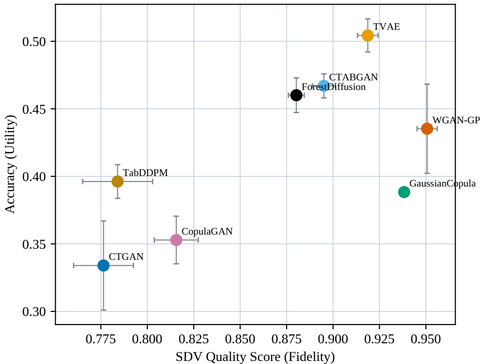
Wine Quality: SDV Quality Score (Fidelity) vs Accuracy (Utility)
